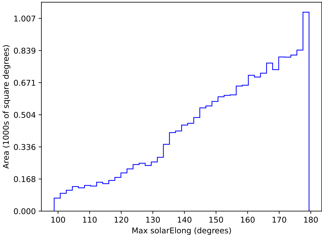
too_elab_r16_d3_giz_v3.4_10yrs WFD z band: Max solarElong
