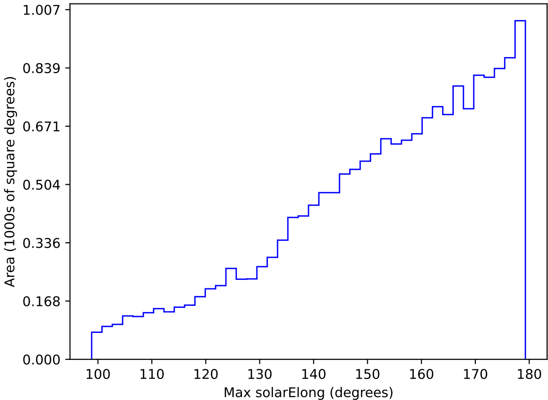
too_elab_r16_d3_giz_v3.4_10yrs WFD y band: Max solarElong
