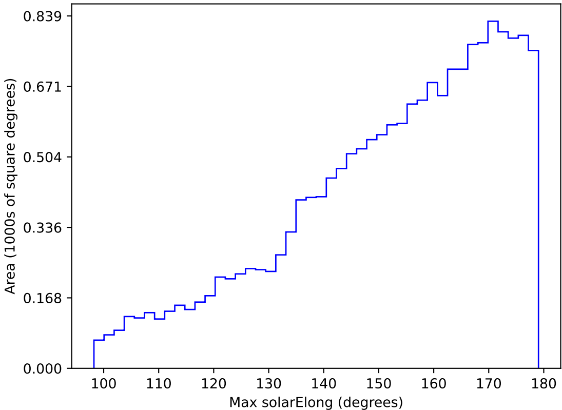
too_elab_r16_d3_giz_v3.4_10yrs WFD u band: Max solarElong
