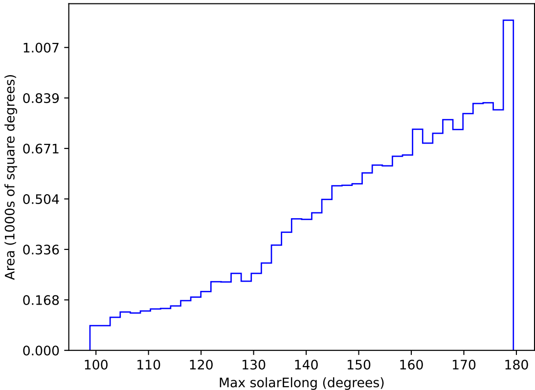
too_elab_r16_d3_giz_v3.4_10yrs WFD r band: Max solarElong
