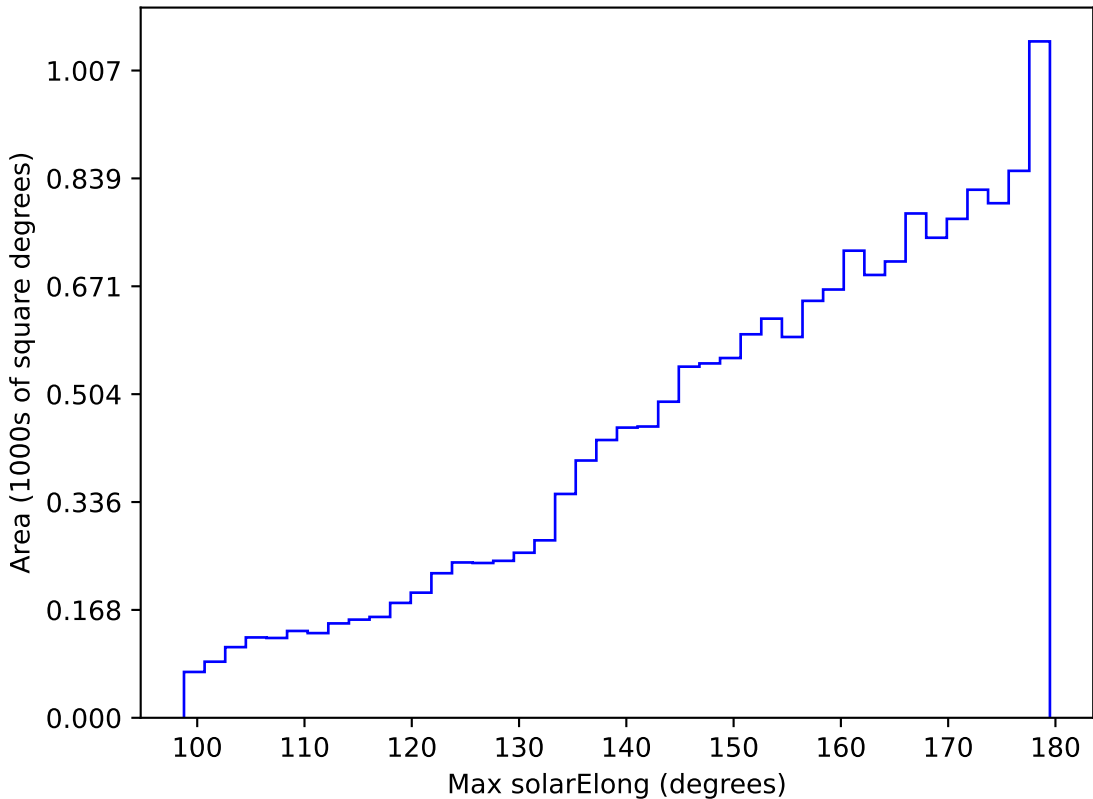
too_elab_r16_d3_giz_v3.4_10yrs WFD i band: Max solarElong
