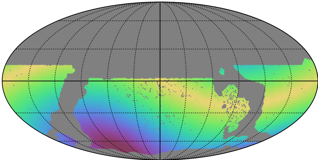
too_elab_r16_d3_giz_v3.4_10yrs WFD g band: Max solarElong
