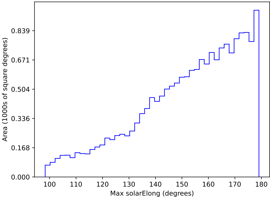
too_elab_r16_d3_giz_v3.4_10yrs WFD g band: Max solarElong
