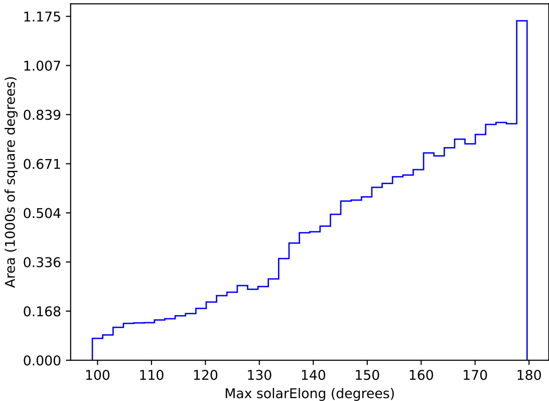
too_elab_r16_d3_giz_v3.4_10yrs WFD all bands: Max solarElong
