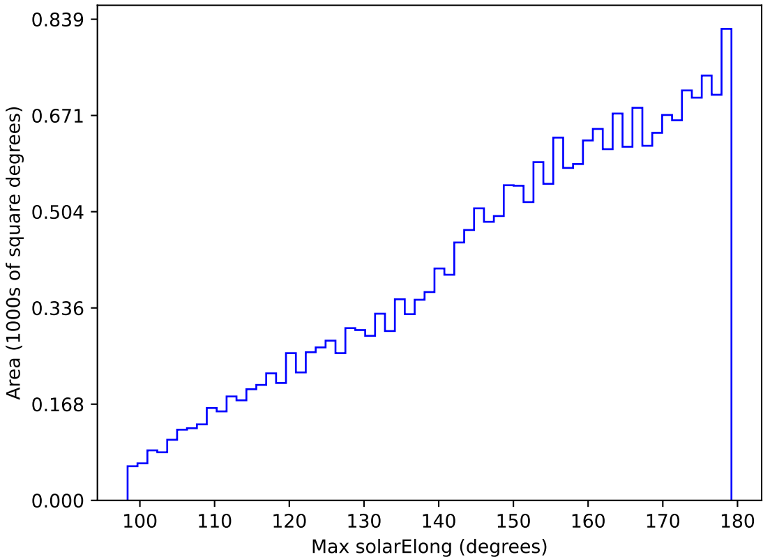
too_elab_r16_d3_giz_v3.4_10yrs All sky y band: Max solarElong
