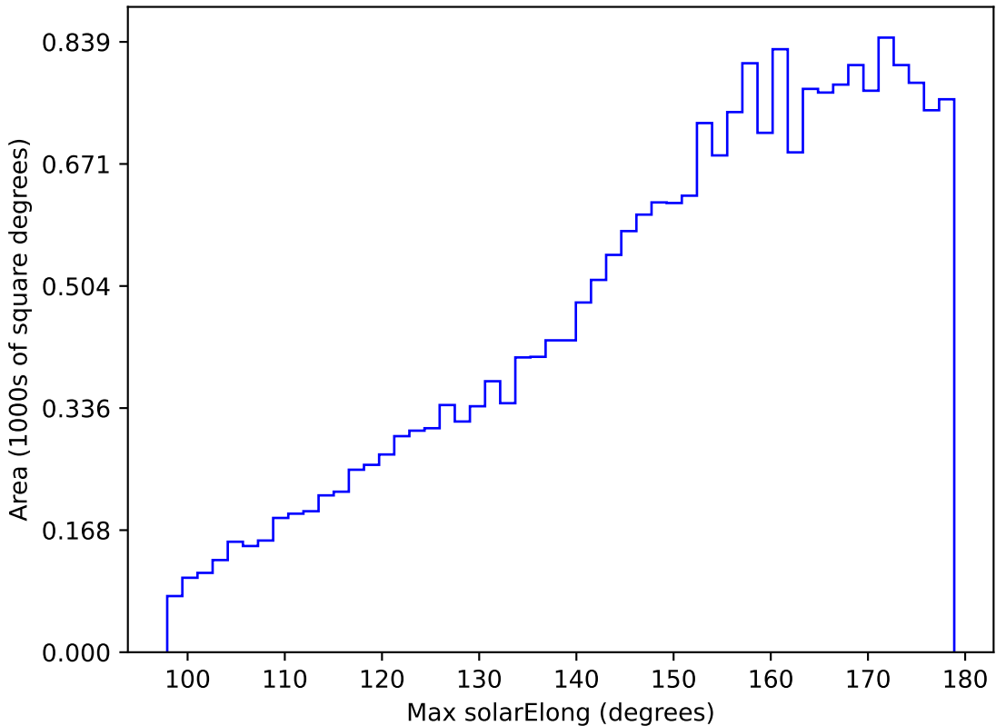
too_elab_r16_d3_giz_v3.4_10yrs All sky u band: Max solarElong
