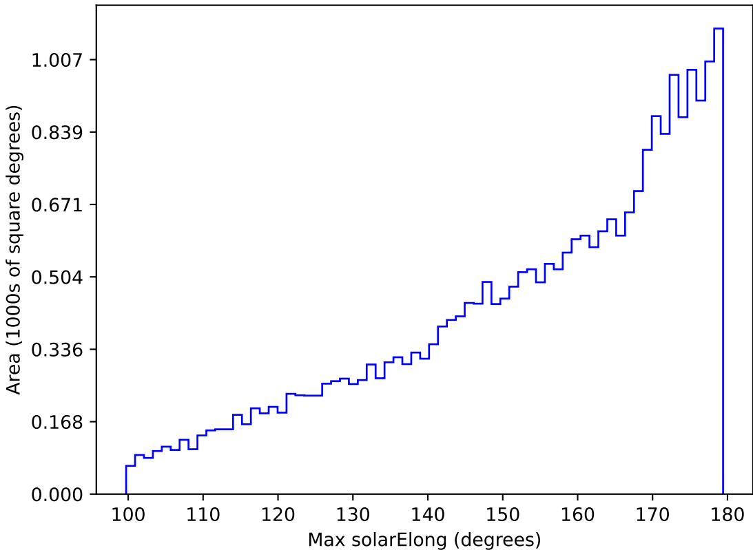
too_elab_r16_d3_giz_v3.4_10yrs All sky r band: Max solarElong
