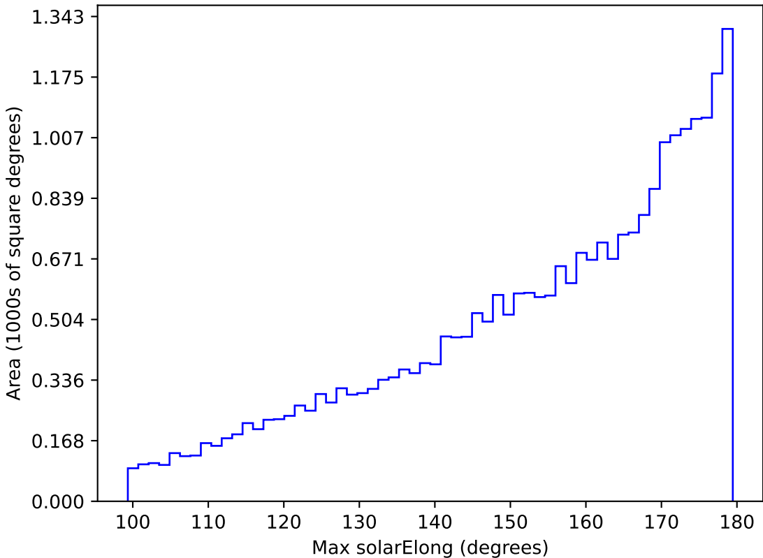
too_elab_r16_d3_giz_v3.4_10yrs All sky i band: Max solarElong
