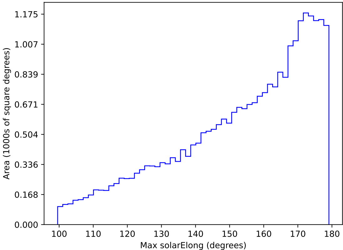
too_elab_r16_d3_giz_v3.4_10yrs All sky g band: Max solarElong
