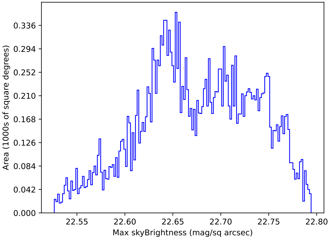
too_elab_r16_d3_giz_v3.4_10yrs Yr 1 u band: Max skyBrightness
