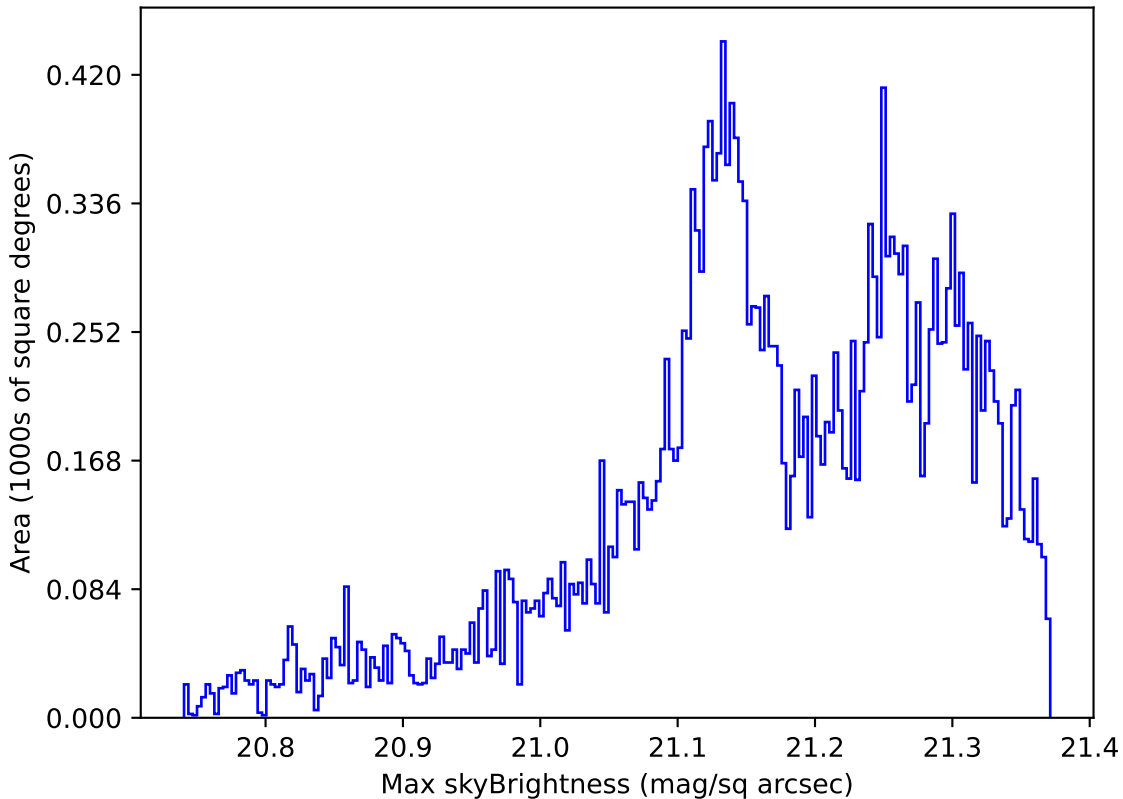
too_elab_r16_d3_giz_v3.4_10yrs Yr 1 r band: Max skyBrightness
