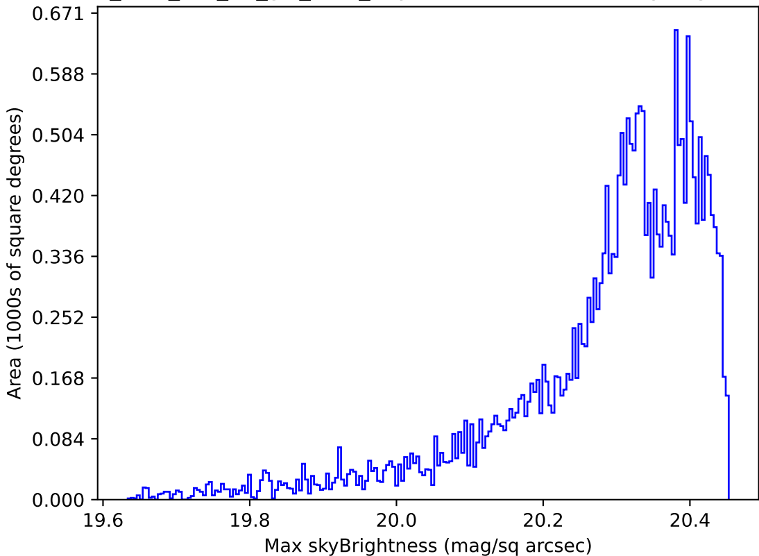
too_elab_r16_d3_giz_v3.4_10yrs Yr 1 i band: Max skyBrightness
