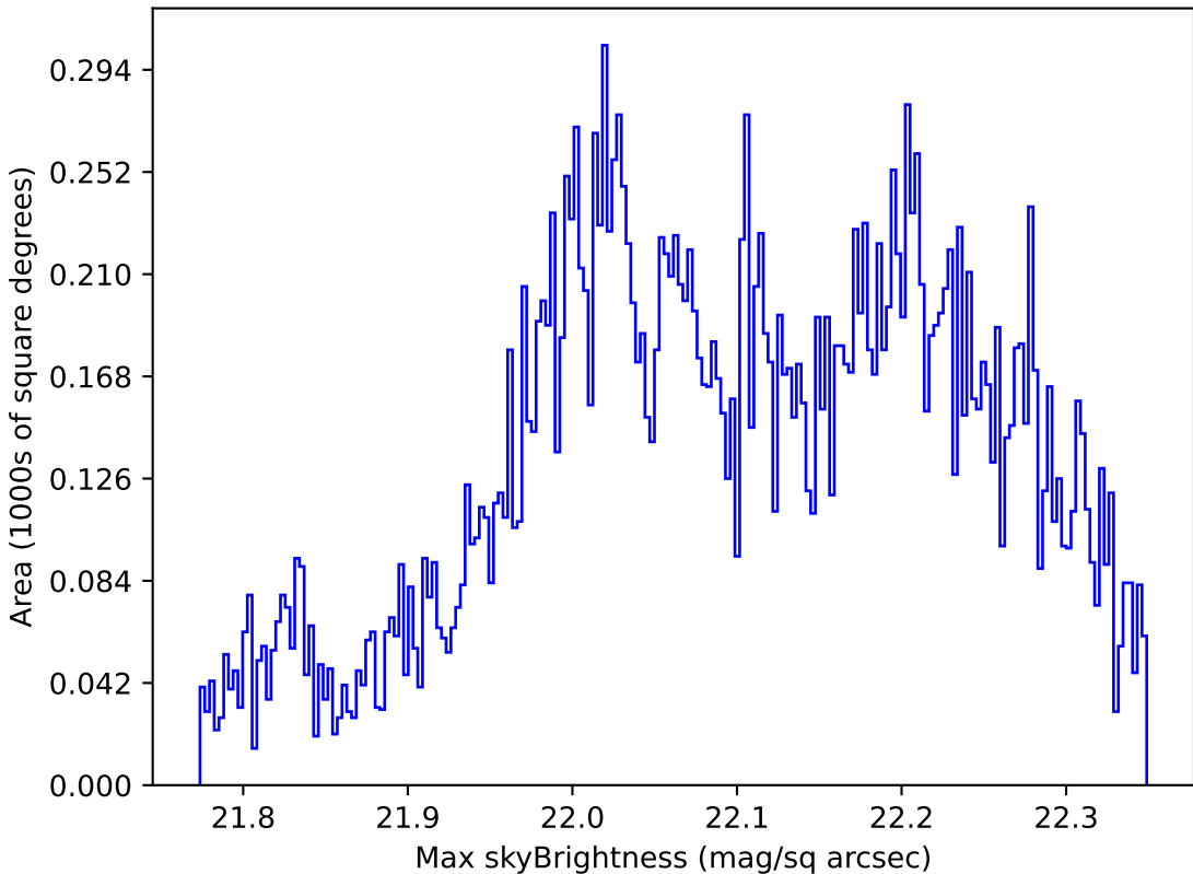
too_elab_r16_d3_giz_v3.4_10yrs Yr 1 g band: Max skyBrightness
