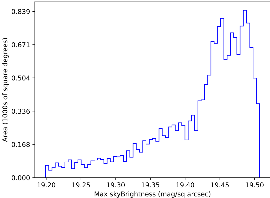
too_elab_r16_d3_giz_v3.4_10yrs WFD z band: Max skyBrightness
