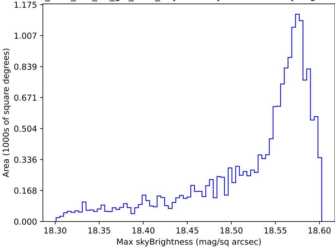
too_elab_r16_d3_giz_v3.4_10yrs WFD y band: Max skyBrightness
