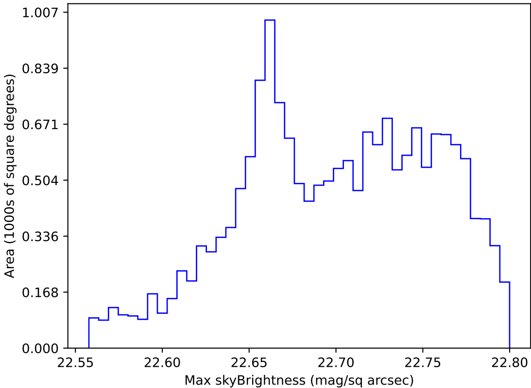
too_elab_r16_d3_giz_v3.4_10yrs WFD u band: Max skyBrightness
