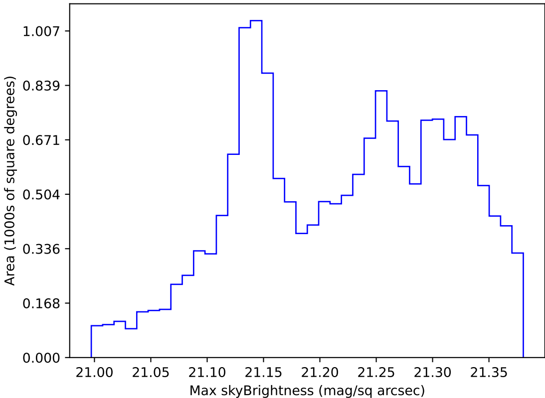
too_elab_r16_d3_giz_v3.4_10yrs WFD r band: Max skyBrightness
