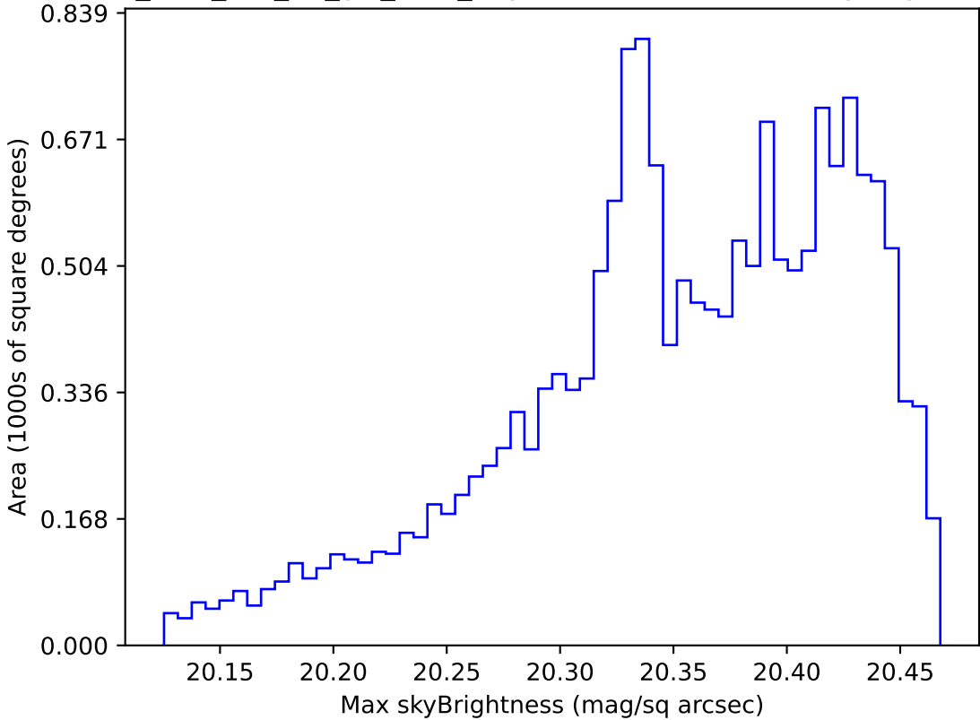
too_elab_r16_d3_giz_v3.4_10yrs WFD i band: Max skyBrightness
