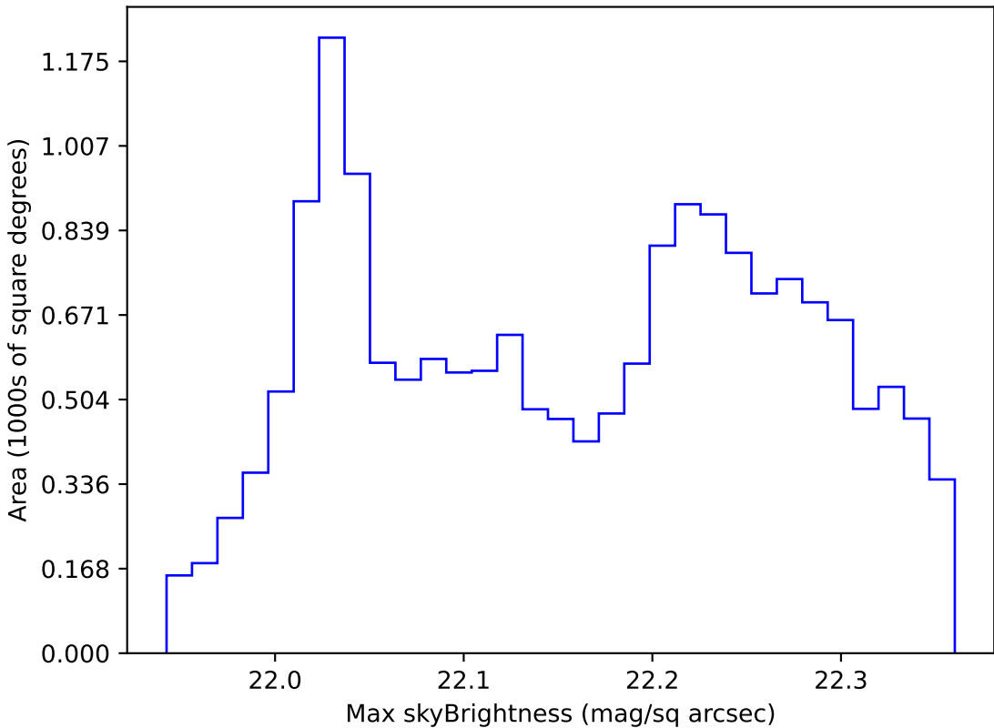
too_elab_r16_d3_giz_v3.4_10yrs WFD g band: Max skyBrightness
