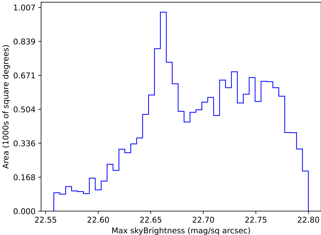
too_elab_r16_d3_giz_v3.4_10yrs WFD all bands: Max skyBrightness
