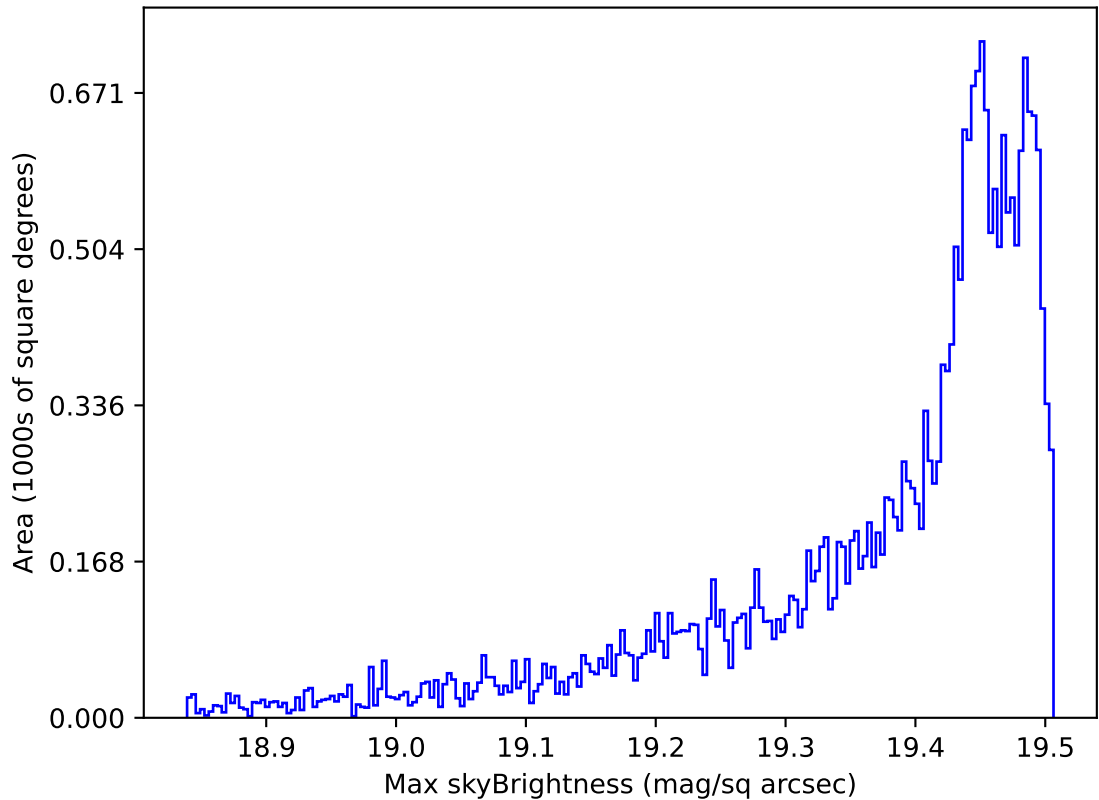
too_elab_r16_d3_giz_v3.4_10yrs All sky z band: Max skyBrightness
