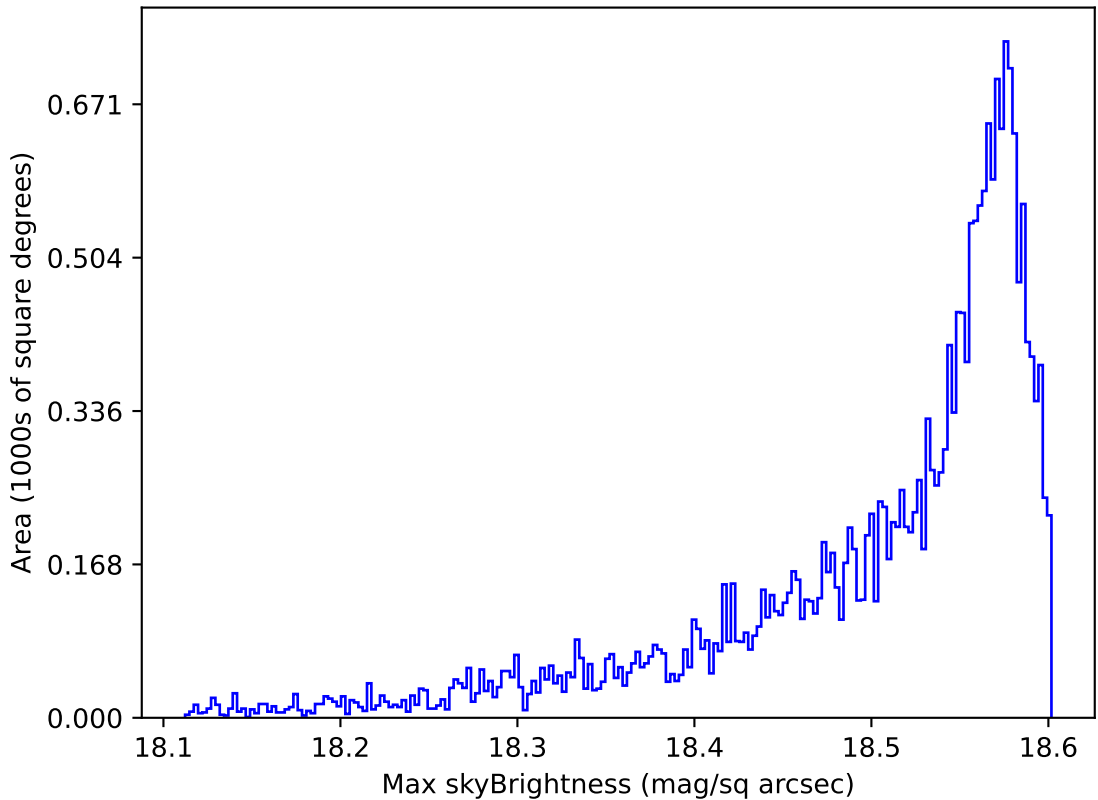
too_elab_r16_d3_giz_v3.4_10yrs All sky y band: Max skyBrightness
