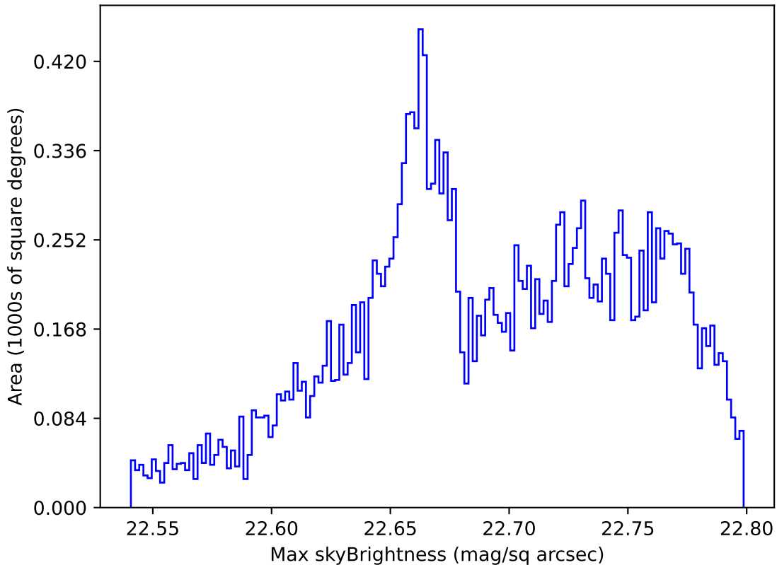
too_elab_r16_d3_giz_v3.4_10yrs All sky u band: Max skyBrightness
