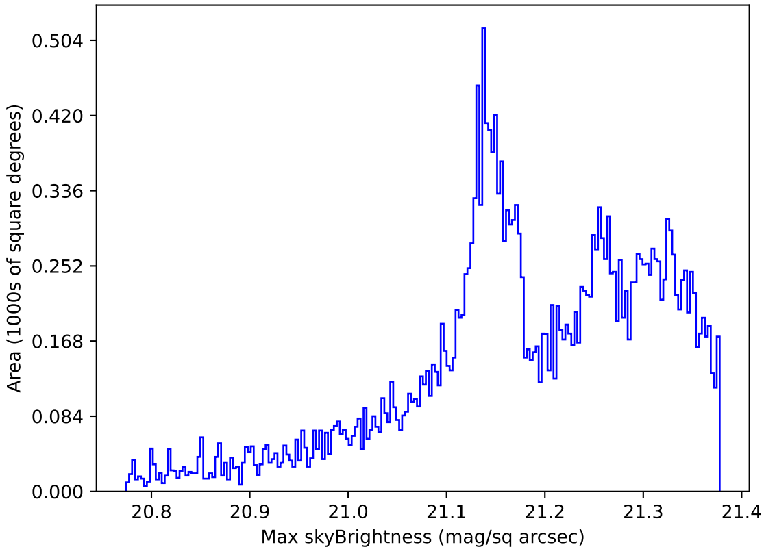
too_elab_r16_d3_giz_v3.4_10yrs All sky r band: Max skyBrightness
