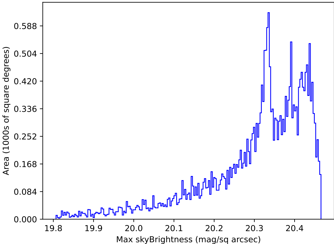
too_elab_r16_d3_giz_v3.4_10yrs All sky i band: Max skyBrightness
