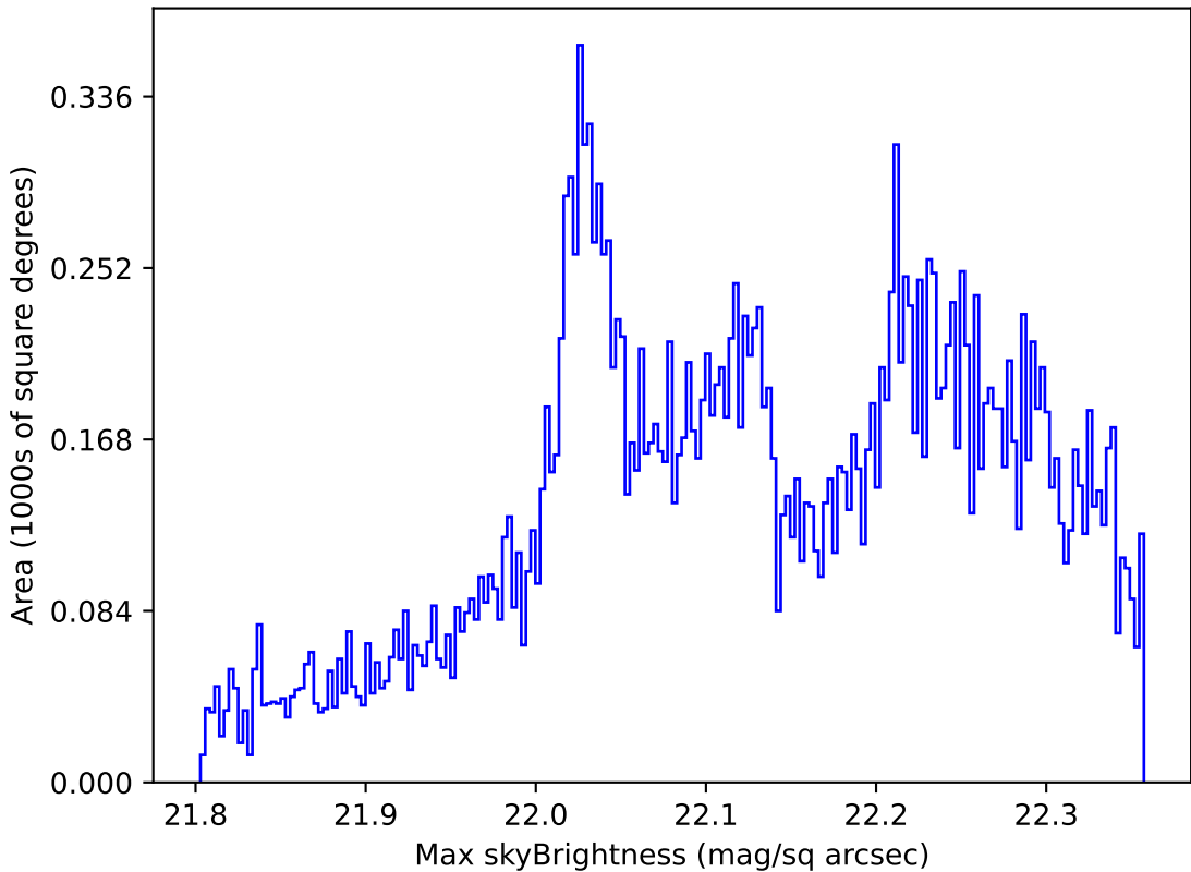
too_elab_r16_d3_giz_v3.4_10yrs All sky g band: Max skyBrightness
