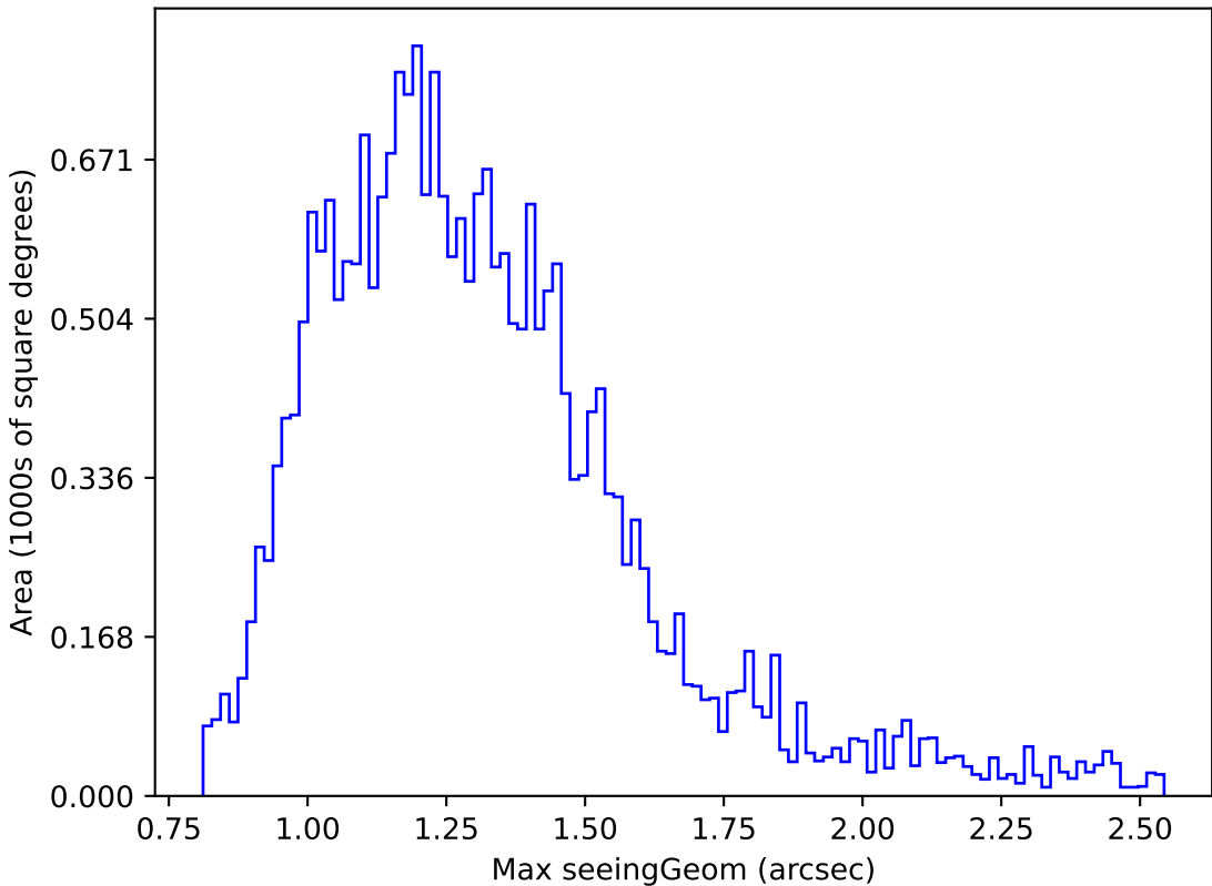
too_elab_r16_d3_giz_v3.4_10yrs Yr 1 z band: Max seeingGeom
