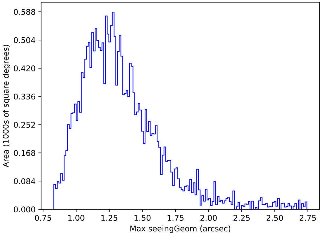
too_elab_r16_d3_giz_v3.4_10yrs Yr 1 u band: Max seeingGeom
