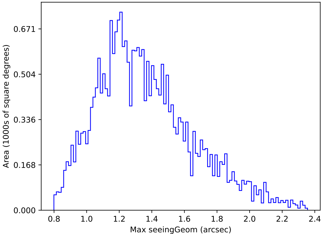
too_elab_r16_d3_giz_v3.4_10yrs Yr 1 r band: Max seeingGeom
