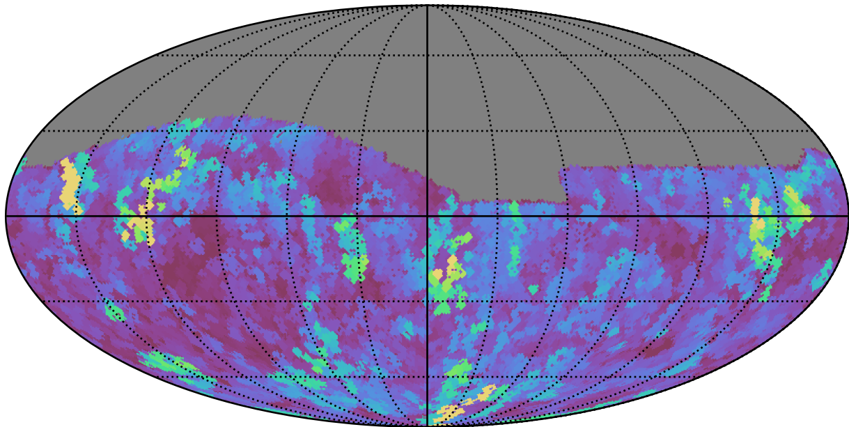
too_elab_r16_d3_giz_v3.4_10yrs Yr 1 i band: Max seeingGeom
