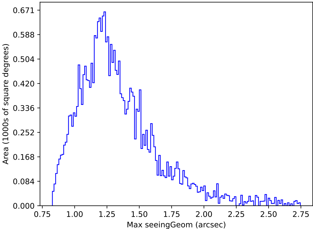
too_elab_r16_d3_giz_v3.4_10yrs Yr 1 i band: Max seeingGeom
