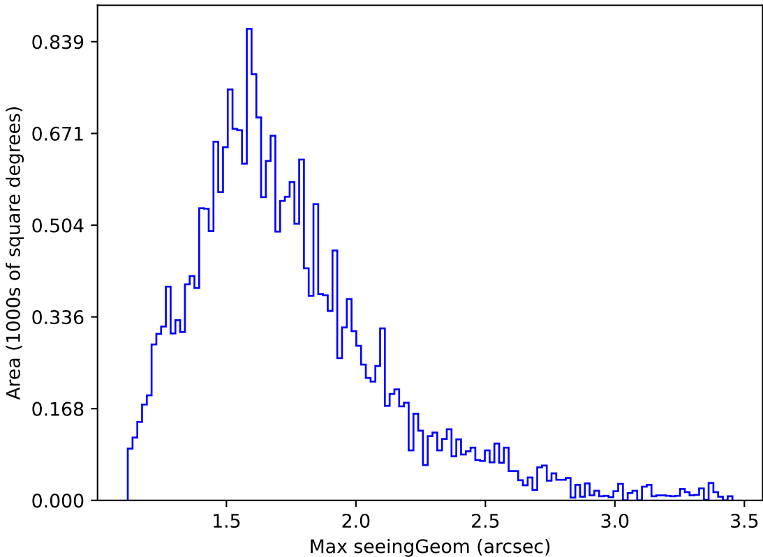
too_elab_r16_d3_giz_v3.4_10yrs Yr 1 all bands: Max seeingGeom
