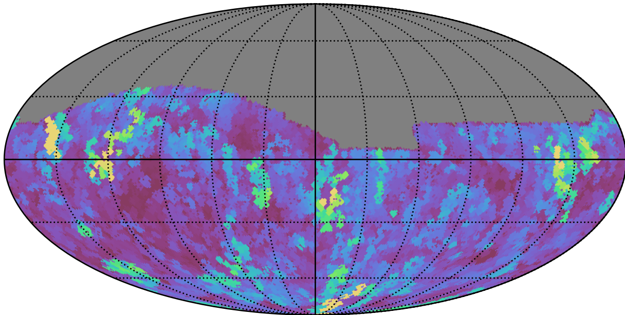
too_elab_r16_d3_giz_v3.4_10yrs Yr 1 i band: Max seeingEff
