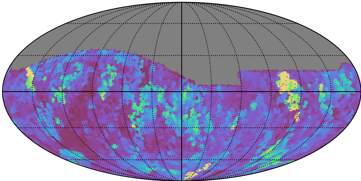
too_elab_r16_d3_giz_v3.4_10yrs Yr 1 all bands: Max seeingEff
