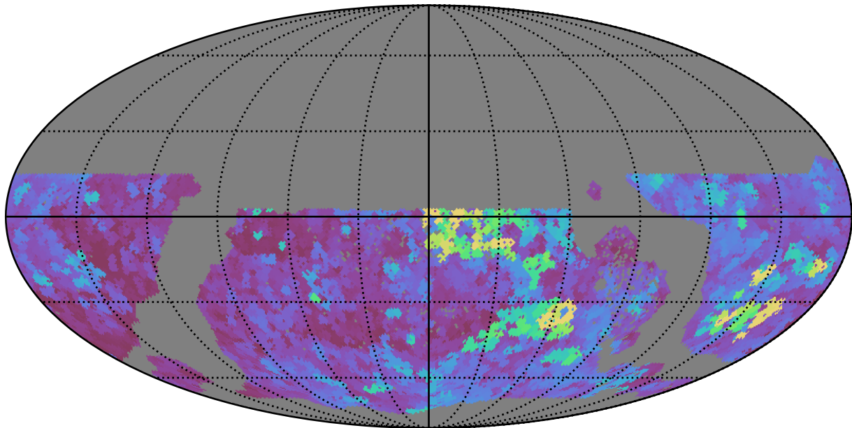
too_elab_r16_d3_giz_v3.4_10yrs WFD y band: Max seeingEff
