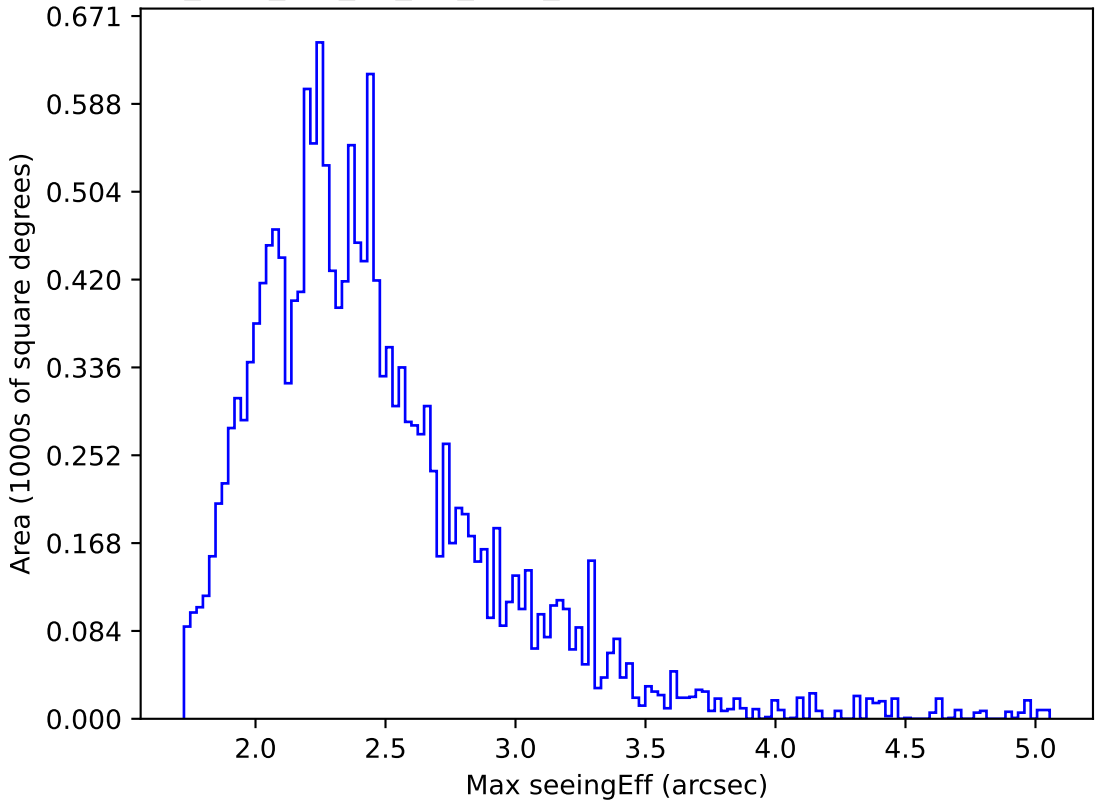
too_elab_r16_d3_giz_v3.4_10yrs WFD u band: Max seeingEff
