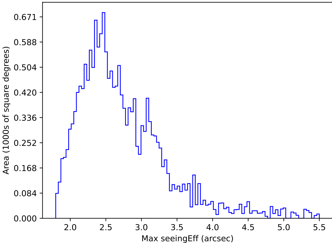
too_elab_r16_d3_giz_v3.4_10yrs WFD i band: Max seeingEff
