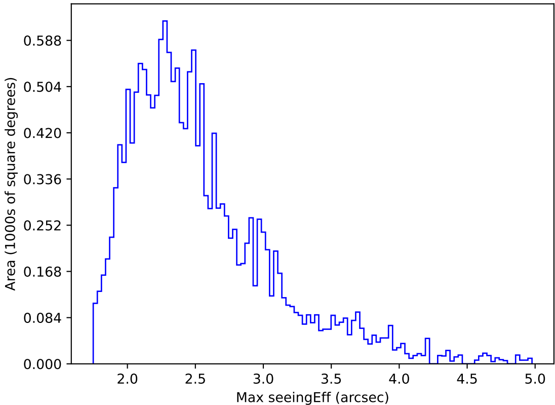
too_elab_r16_d3_giz_v3.4_10yrs WFD g band: Max seeingEff
