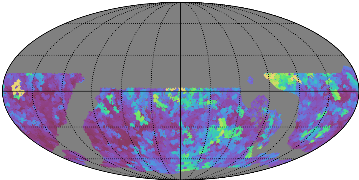
too_elab_r16_d3_giz_v3.4_10yrs WFD all bands: Max seeingEff
