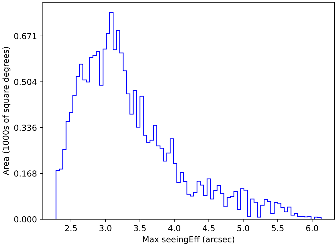
too_elab_r16_d3_giz_v3.4_10yrs WFD all bands: Max seeingEff
