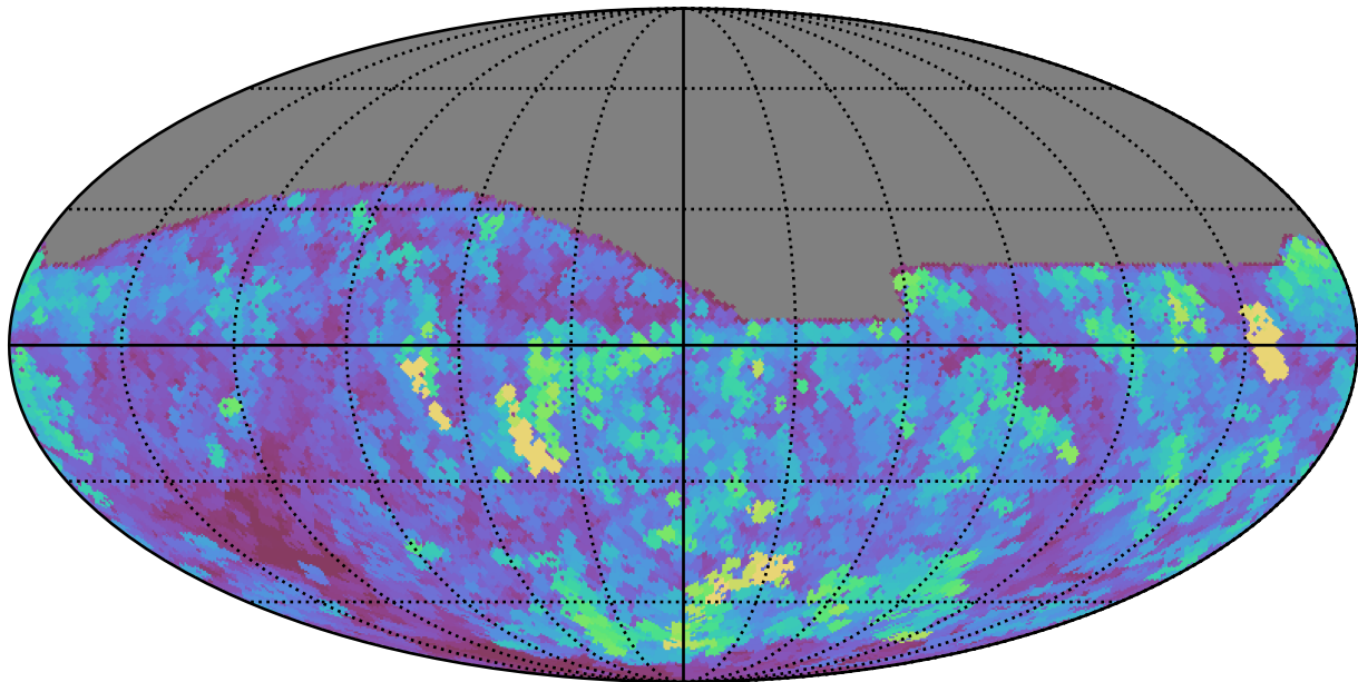
too_elab_r16_d3_giz_v3.4_10yrs All sky z band: Max seeingEff
