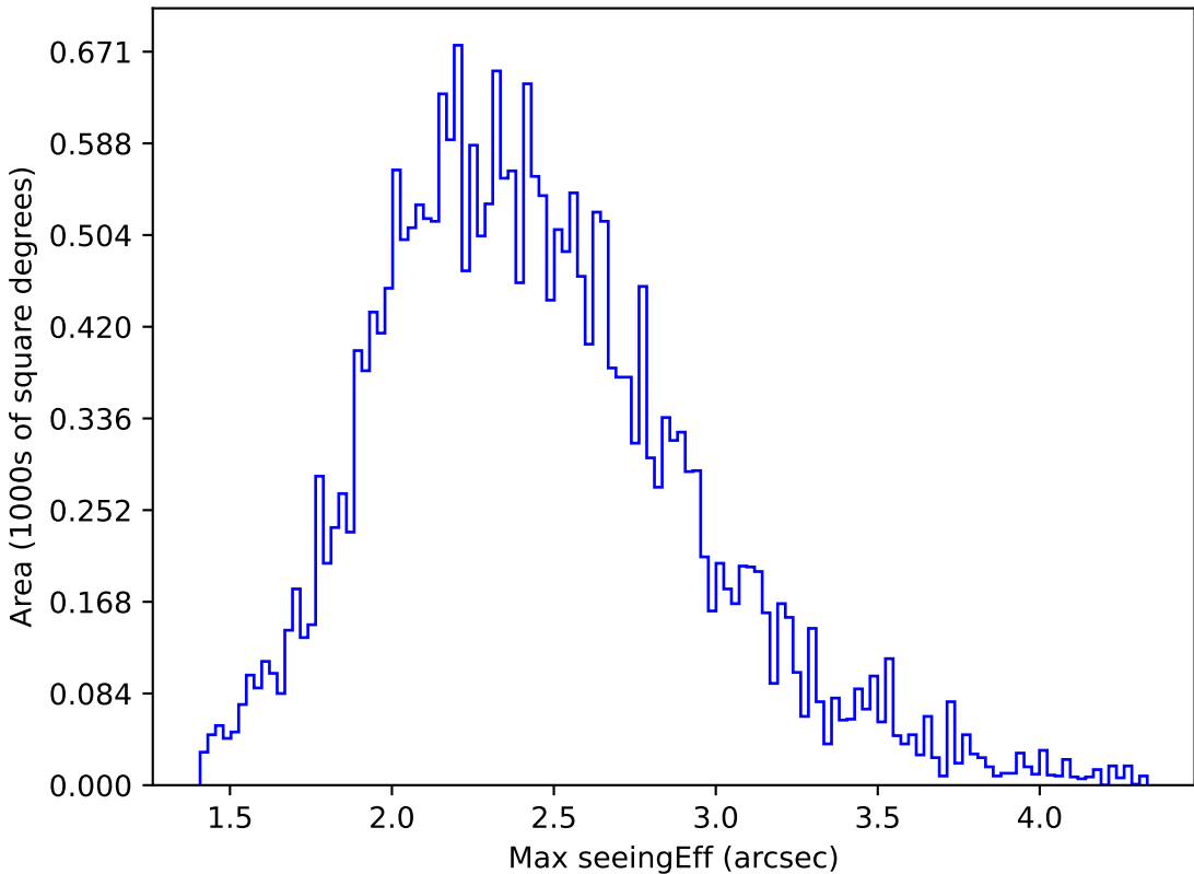
too_elab_r16_d3_giz_v3.4_10yrs All sky z band: Max seeingEff
