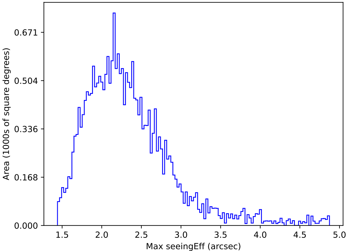
too_elab_r16_d3_giz_v3.4_10yrs All sky y band: Max seeingEff
