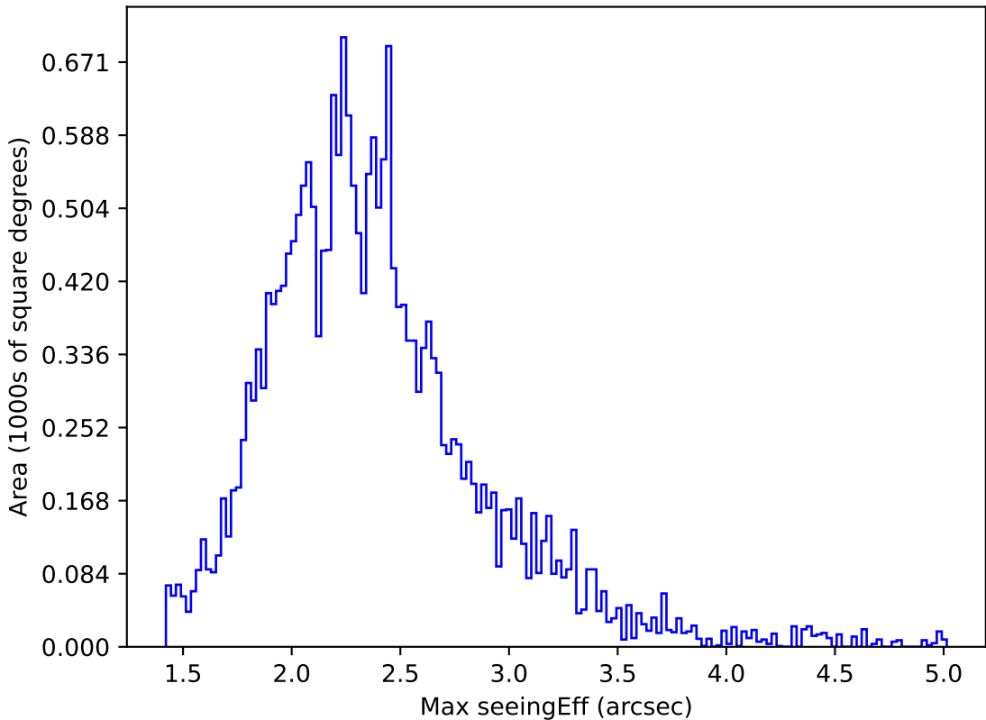
too_elab_r16_d3_giz_v3.4_10yrs All sky u band: Max seeingEff
