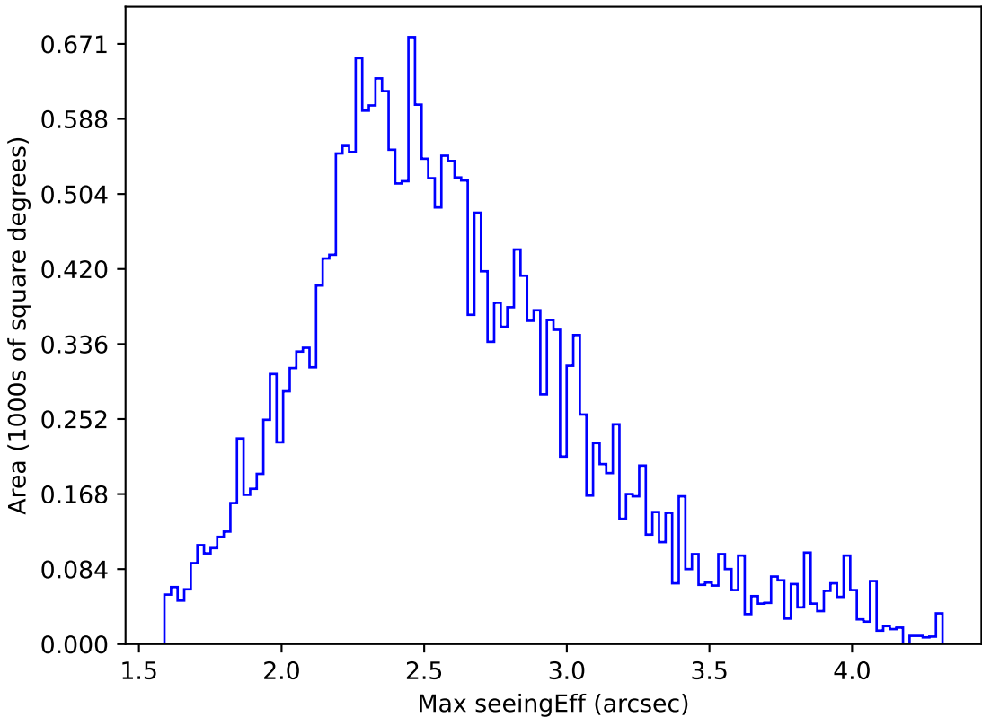
too_elab_r16_d3_giz_v3.4_10yrs All sky r band: Max seeingEff
