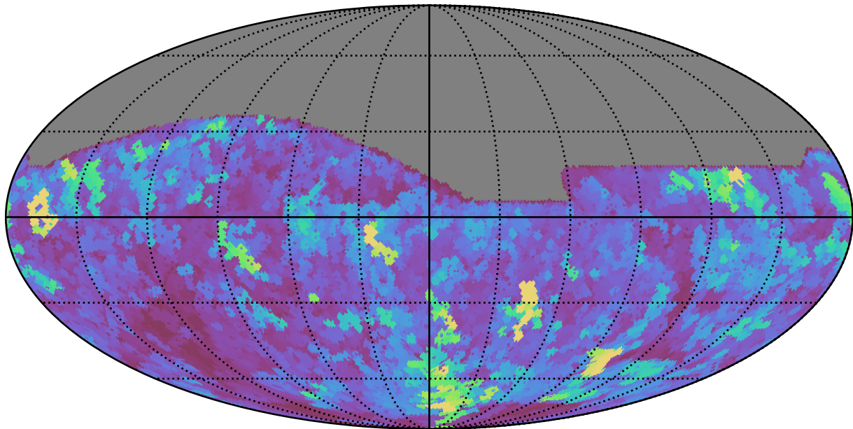
too_elab_r16_d3_giz_v3.4_10yrs All sky i band: Max seeingEff
